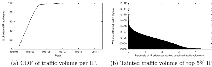
Fig. 5: Tainted traffic to/from internal IP addresses.
