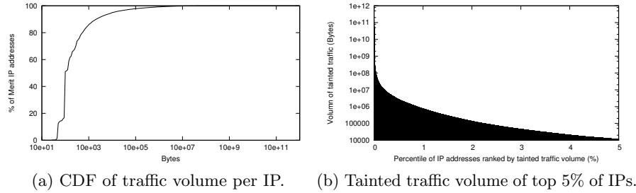
Fig. 4: Tainted traffic to/from external IP addresses.
