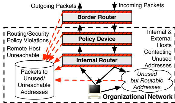
Figure 1: Unused and unreachable addresses inside a network. These addresses can come from a range of sources including routing and policy enforcement devices.
